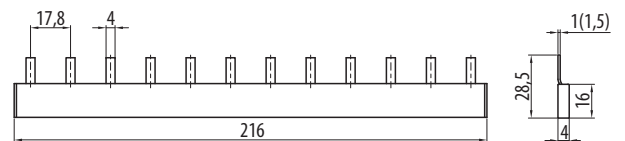
S1L-210-10, S1L-210-16
