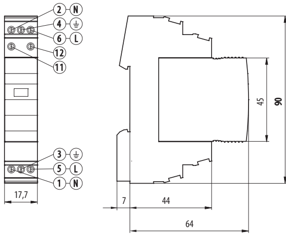
SVD-253-1N-MZS
